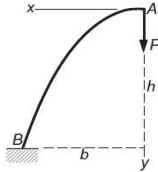
Figura 4.1: Cantilever semiparabolic
